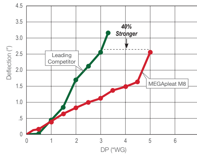
Results from a wet breach test performed at an independent test lab shows the MEGApleat® M8 filter is over 40% stronger than the leading competitor.
