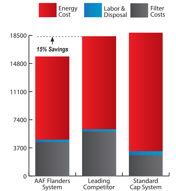
Analysis based on a 3-stage filter system, running 20,000 CFM, over a 2 year time period. Energy costs based on the national average of 0.08 $/kW-hr. Filter selection was based on the most energy efficient filters available.
