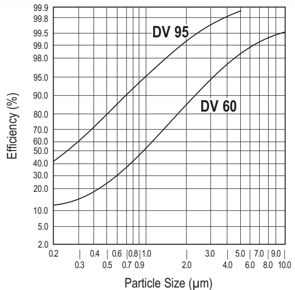
Efficiency By Particle Size
